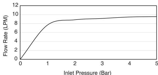
Flow Curve (K-26293T)
