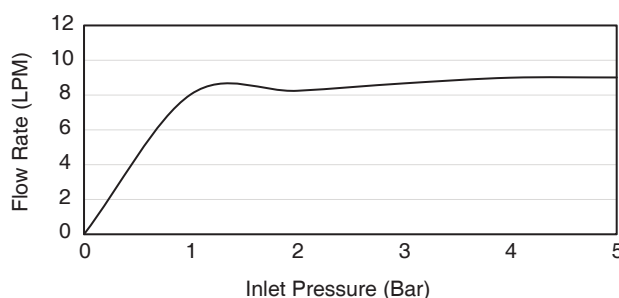
Flow Curve (K-26294T)
