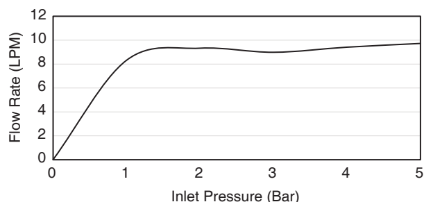
Flow Curve (K-26292T)
