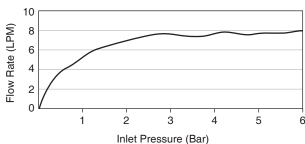
Flow Curve
