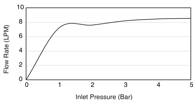
Flow Curve Handshower for BL
