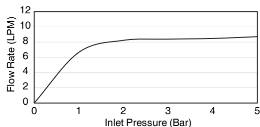
Flow Curve (Rain mode)
