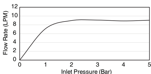
Flow Curve (Waterfall mode)
