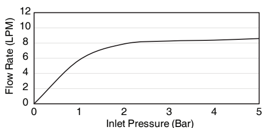
Flow Curve (Moving spray mode)
