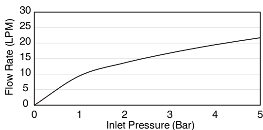
Flow Curve (1 Outlet)
