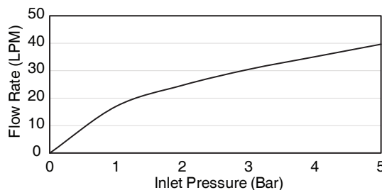
Flow Curve (2 Outlet)
