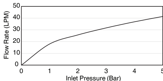
Flow Curve (3 Outlet)
