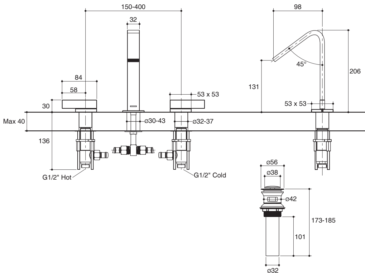
Product Diagram
