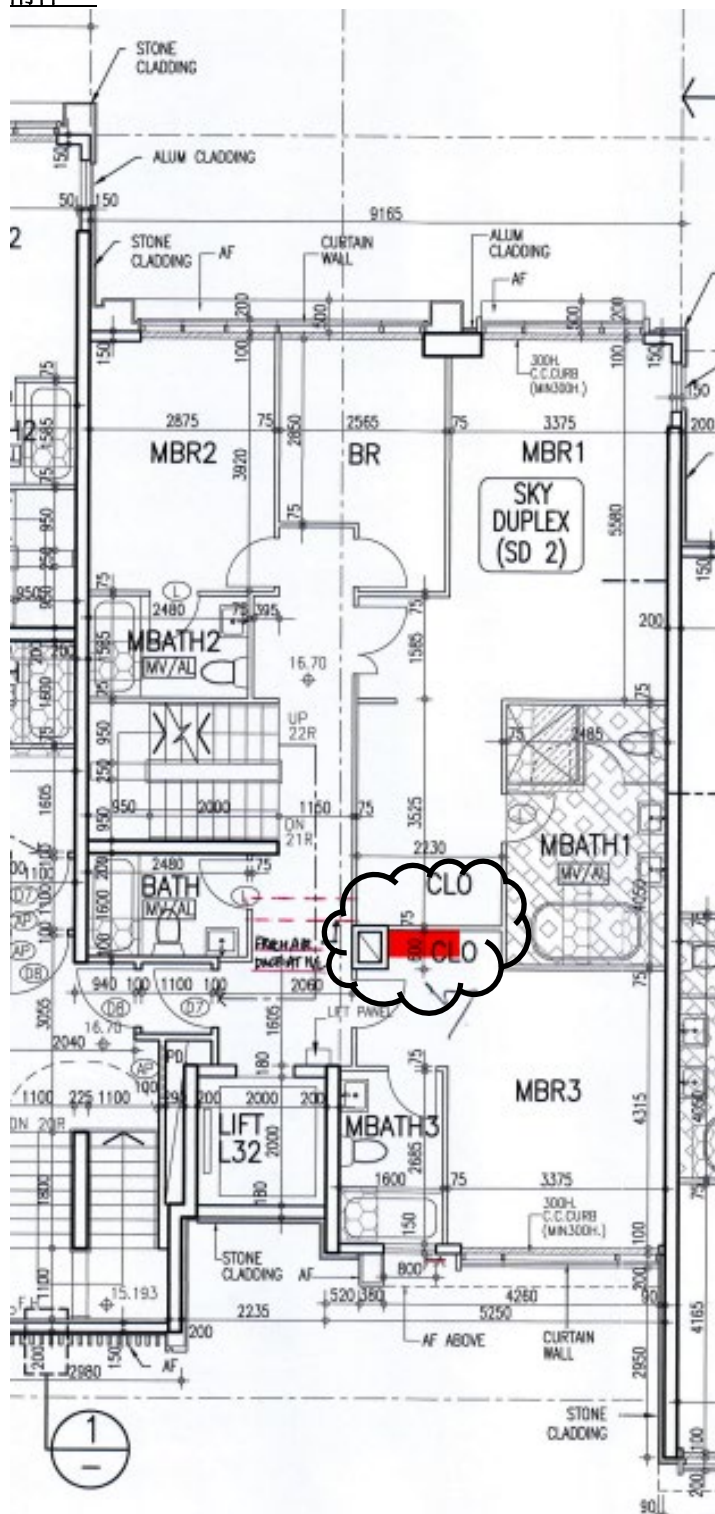
Image 2 : Part Plan of Block H1, Sky Duplex (SD 2)- 3/F extracted from mark-up plan on approved General Building Plan (GBP) (amendment no. 13) dated May 07, 2020, drawing number A-47 Revision M. In compare of Image 1 and Image 2 , Part plan of Block H1, Sky Duplex (SD 2)- 3/F, change of layout (amendment no. 13) is clouded for reference. Furring wall (with 950x200mm at MBR3-CLO) is added on plan.
