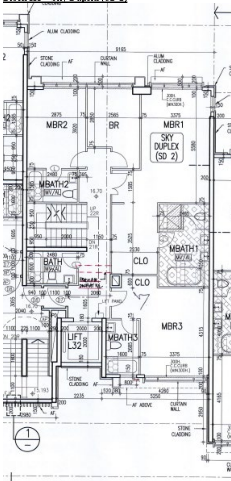
Image 1: Part Plan of Block H1, Sky Duplex (SD 2)- 3/F extracted from approved General Building Plan (GBP) (amendment no. 13) dated May 07, 2020, drawing number A-47 Revision M.
