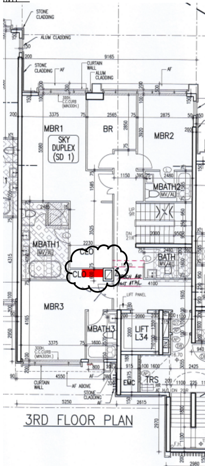
Image 2 : Part Plan of Block H2, Sky Duplex (SD 1)- 3/F extracted from mark-up plan on approved General Building Plan (GBP) (amendment no. 13) dated May 07, 2020, drawing number A-47 Revision M. In compare of Image 1 and Image 2 , Part plan of Block H2, Sky Duplex (SD 1)- 3/F, change of layout (amendment no. 13) is clouded for reference. Furring wall (with 1000x200mm at MBR3-CLO) is added on plan.
