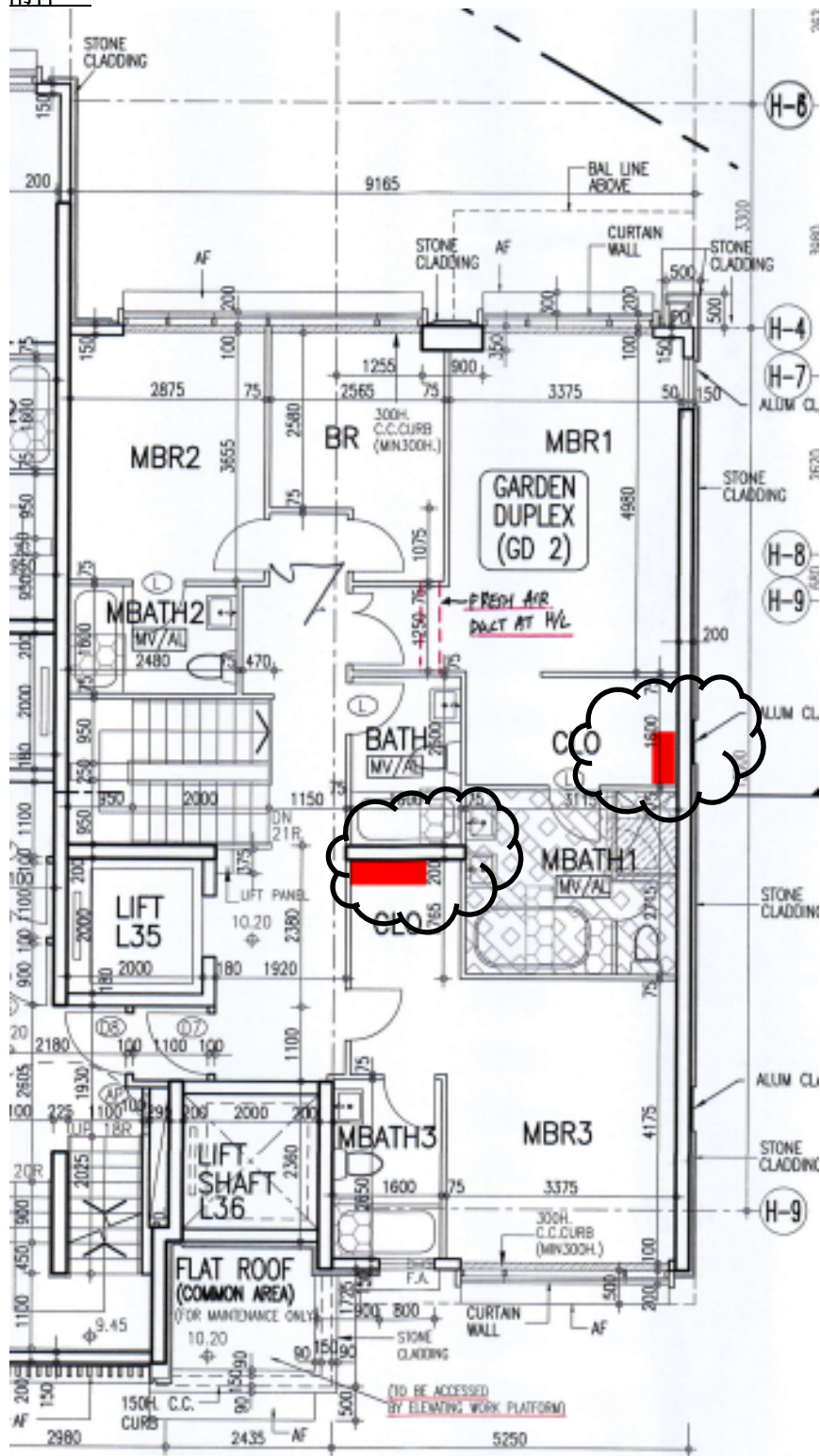
Image 2: Part Plan of Block H2, Garden Duplex (GD 2)- 1/F extracted from mark-up plan on approved General Building Plan (GBP) (amendment no. 13) dated May 07, 2020, drawing number A-46 Revision M. In compare of Image 1 and Image 2 , Part plan of Block H2, Garden Duplex (GD 2)- 1/F, change of layout (amendment no. 13) is clouded for reference. Furring walls (with 800x200mm at MBR1-CLO& 700x200mm at MBR3-CLO) is added on plan.
