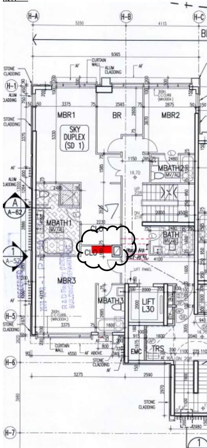
Image 2 : Part Plan of Block H1, Sky Duplex (SD 1)- 3/F extracted from mark-up plan on approved General Building Plan (GBP) (amendment no. 13) dated May 07, 2020, drawing number A-47 Revision M. In compare of Image 1 and Image 2 , Part plan of Block H1, Sky Duplex (SD 1)- 3/F, change of layout (amendment no. 13) is clouded for reference. Furring wall (with 1000x200mm at MBR3-CLO) is added on plan.
