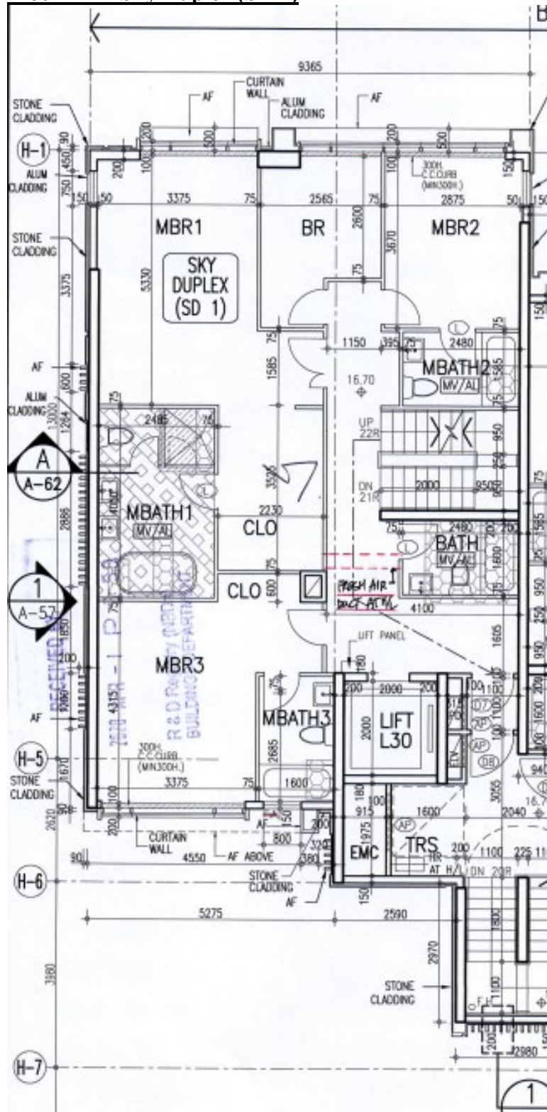
Image 1: Part Plan of Block H1, Sky Duplex (SD 1)- 3/F extracted from approved General Building Plan (GBP) (amendment no. 13) dated May 07, 2020, drawing number A-47 Revision M.
