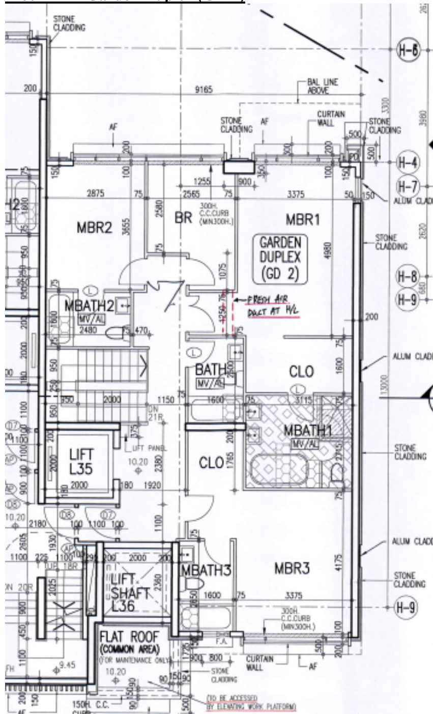
Image 1: Part Plan of Block H2, Garden Duplex (GD 2)- 1/F extracted from approved General Building Plan (GBP) (amendment no. 13) dated May 07, 2020, drawing number A-46 Revision M.
