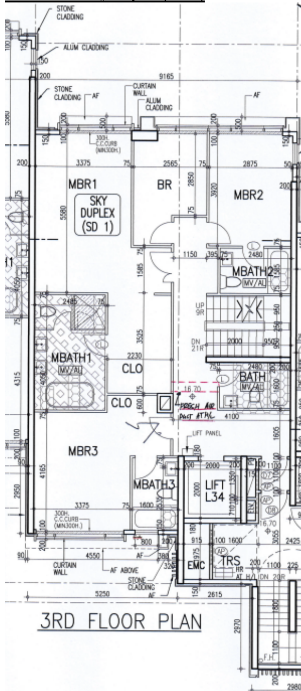
Image 1: Part Plan of Block H2, Sky Duplex (SD 1)- 3/F extracted from approved General Building Plan (GBP) (amendment no. 13) dated May 07, 2020, drawing number A-47 Revision M.
