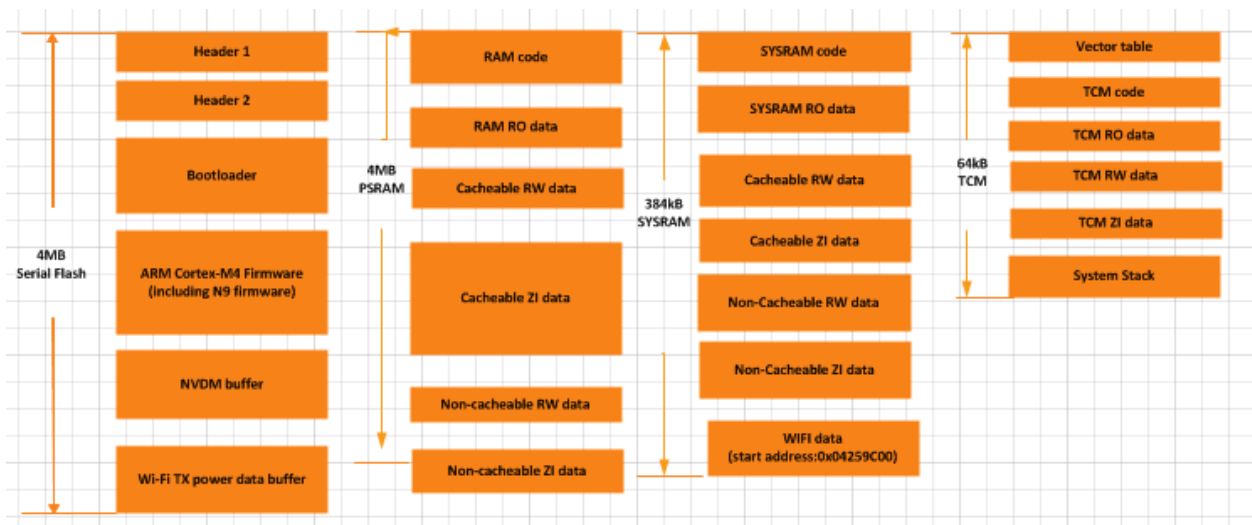
Figure 21. Execution view of the MT7686D memory layout without FOTA
