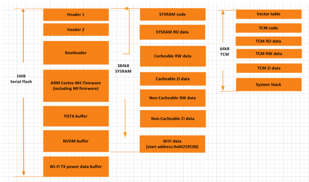
Figure 17. Execution view of the MT7682S memory layout with full binary FOTA
