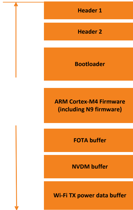
Figure 22. Load view of the MT7686D memory layout with full binary FOTA
