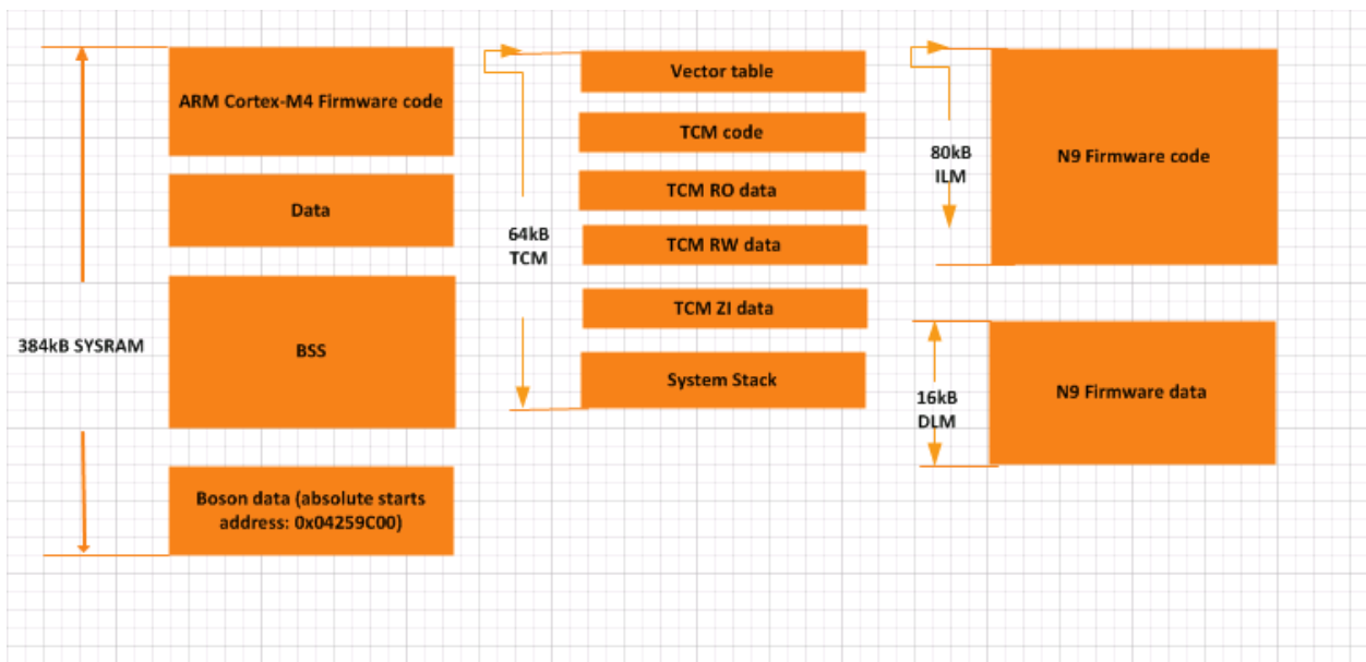
Figure 25 MT5932 execution view memory layout without external flash
