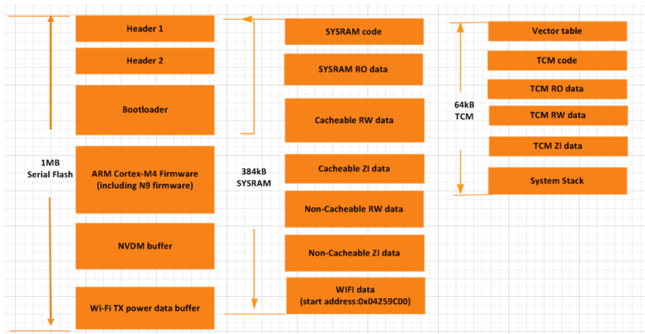
Figure 15. Execution view of the MT7682S memory layout without FOTA
