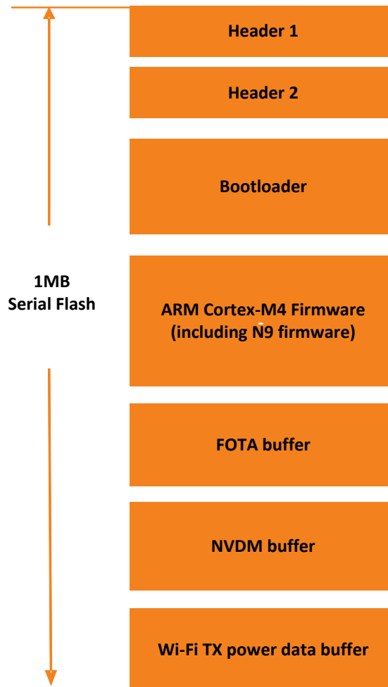
Figure 16. Load view of the MT7682S memory layout with full binary FOTA
