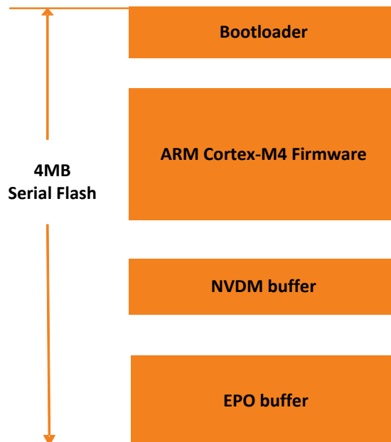
Figure 6. Load view of the MT2523D and MT2523G memory layout without FOTA
