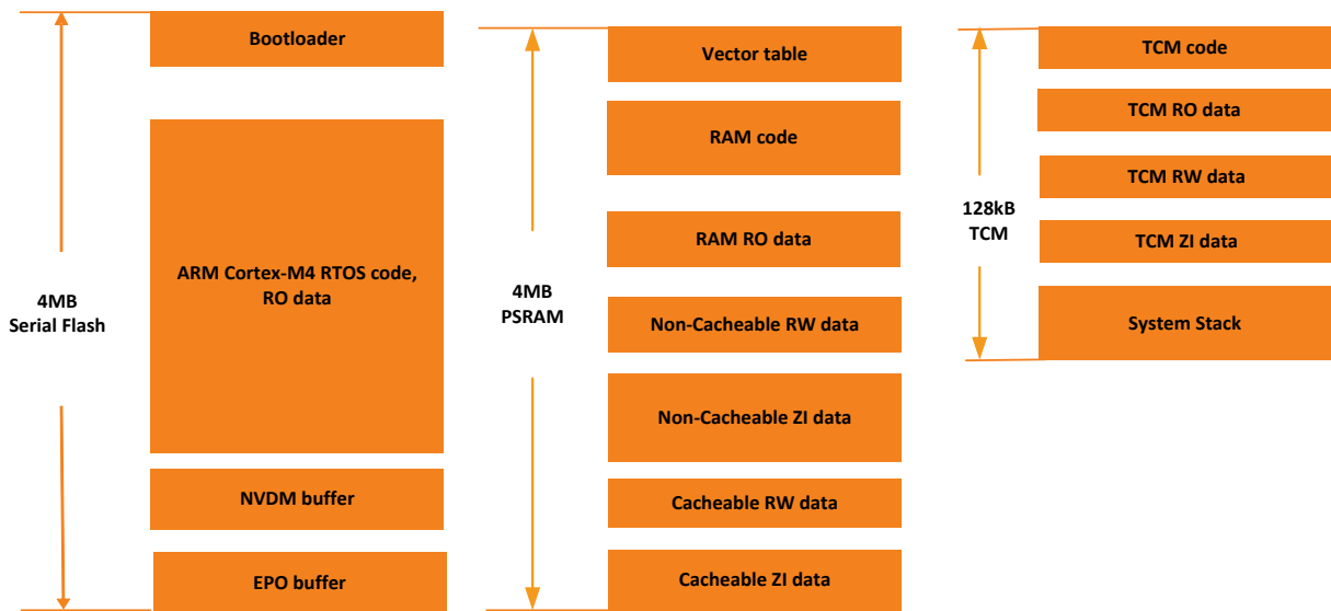
Figure 8. Execution view of the MT2523D, MT2523G and MT2533 memory layout without FOTA
