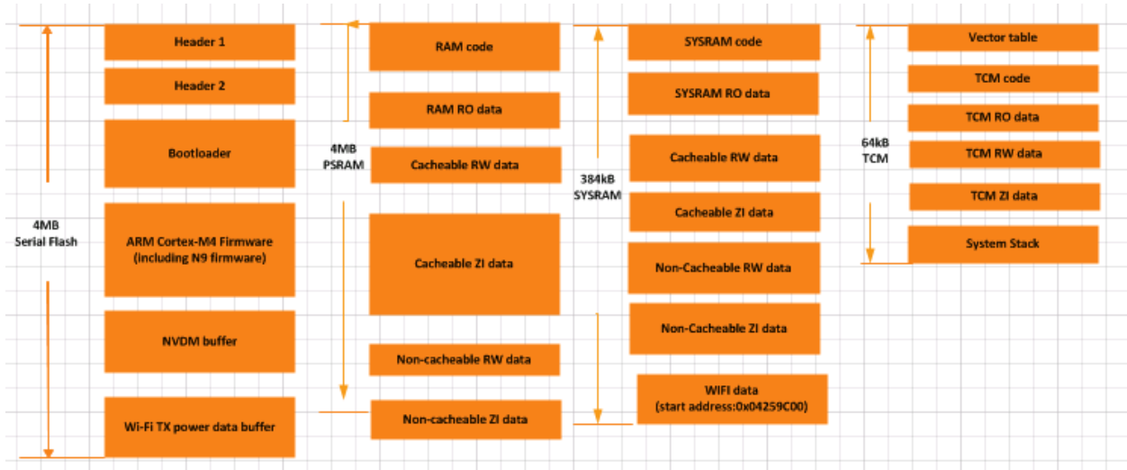
Figure 23. Execution view of the MT7682S memory layout with full binary FOTA
