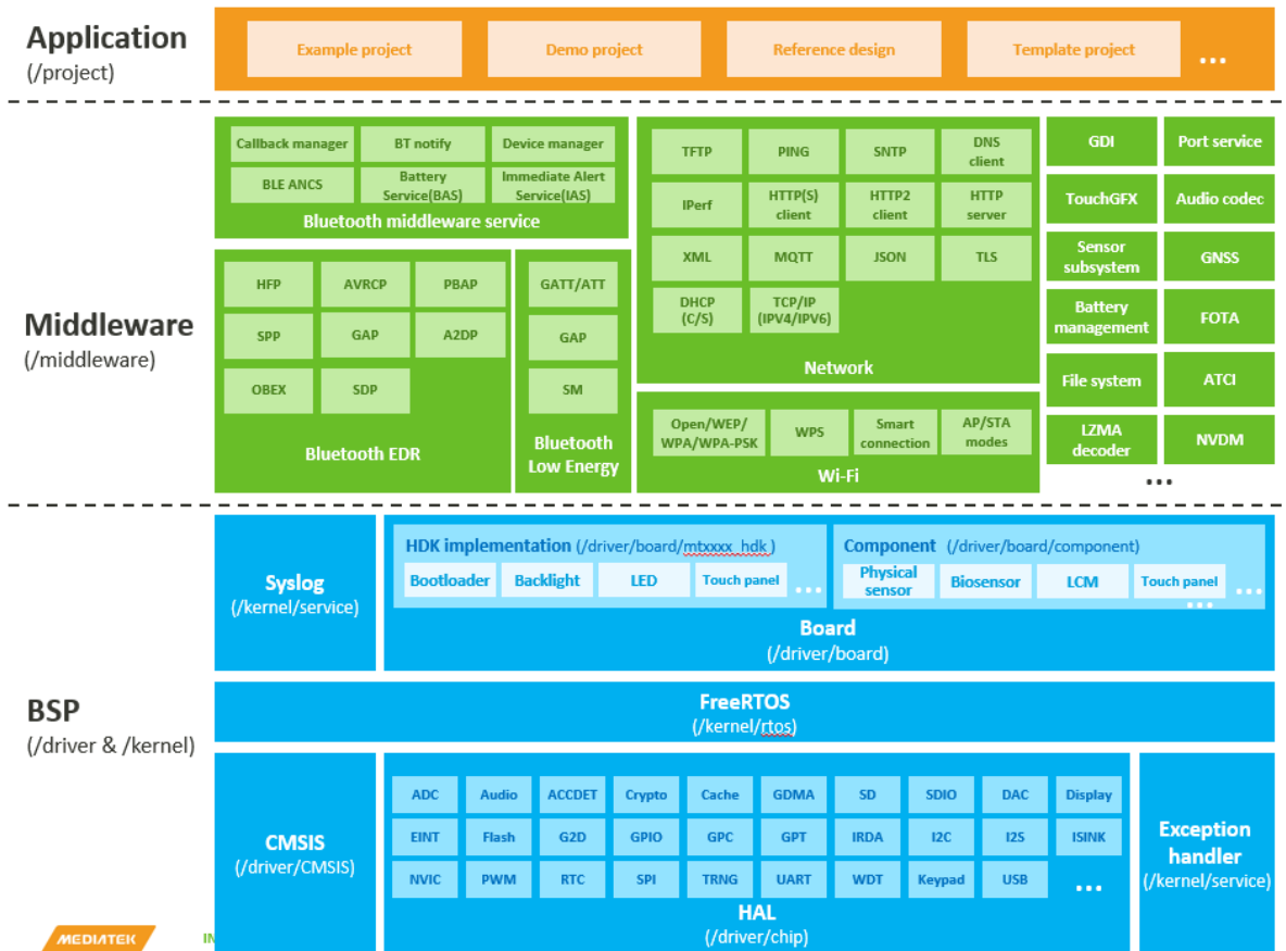
Figure 1. Software architecture
