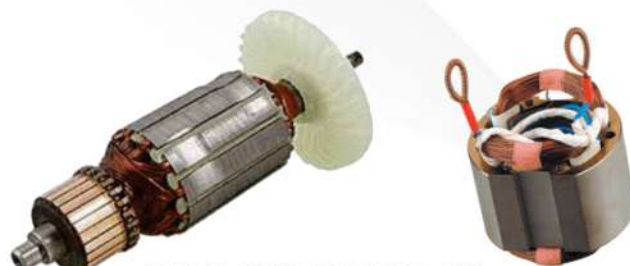
CM-4 SB ARMATURE & FIELD COIL
