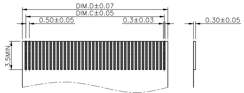
FPC LAYOUT SCALE 3.2/1
